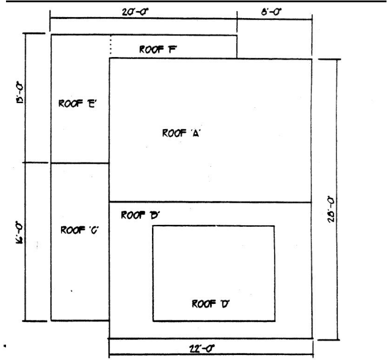
ROOF PLAN
